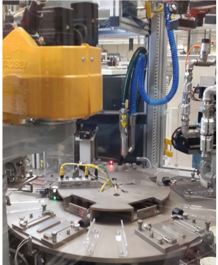
Microscan's Vision HAWK is integrated into a robot arm for vision inspection on the assembly line.
