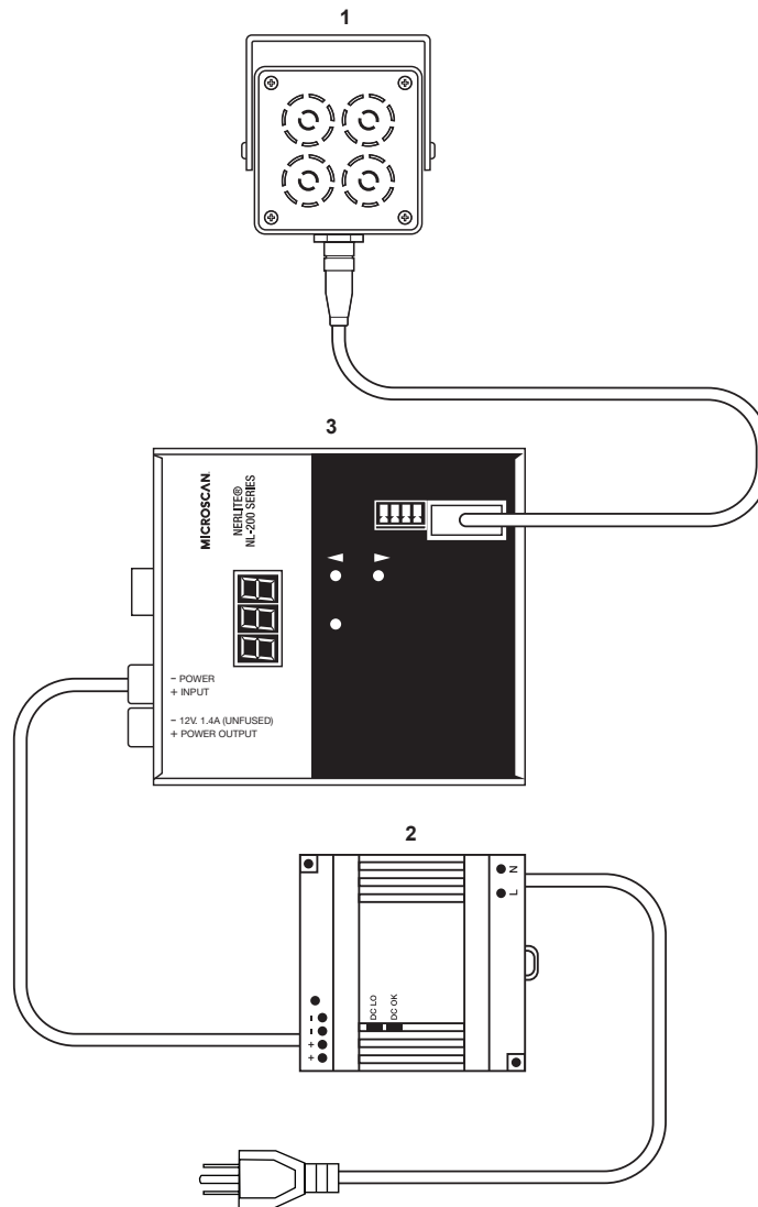
Figure A LALL Series Illuminator with NL-200 Controller and power supply
