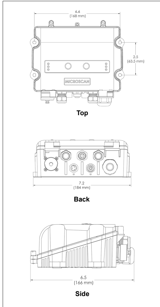
MS-Connect 210 Dimensions
